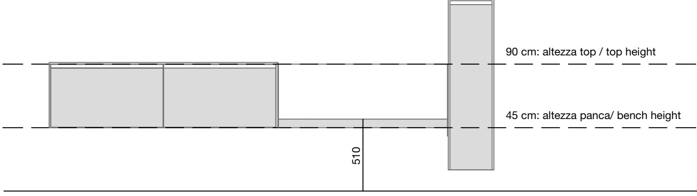
BASI - CABINETS H45
