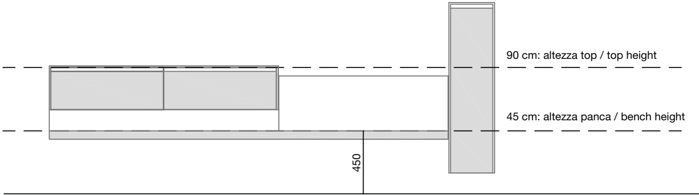
BASI H30 CON MENSOLA INFERIORE CABINETS H30 WITH LOWER SHELF
