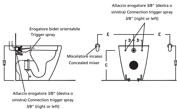
Vaso filo muro -Wc back-to-wall-Stand Wc
