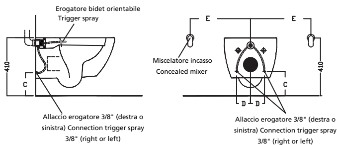
Vaso Sospeso -Wall-hung WC-Hang Wc
