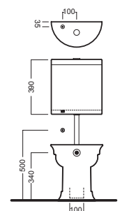
Entrata acqua bassa (sx) Bottom water inlet (left)
