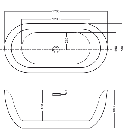
vasca 170x78 BT_01 bathtub 170x78 BT_01
