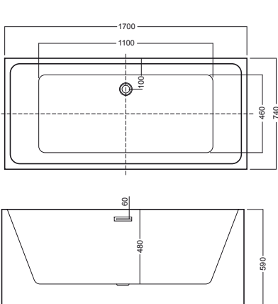
vasca 170x74 BT_02 bathtub 170x74 BT_02
