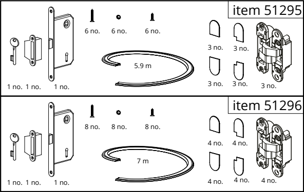
60 kg hinge set + keyed lock and electric striker
