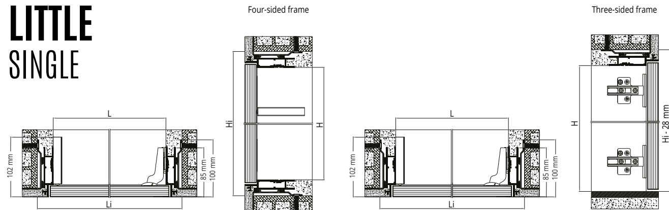
Single Door - Non-Std Size - Three-sided frame
