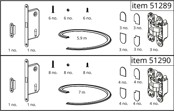
60 kg hinge set + deadlocks for fixed-leaf double door
