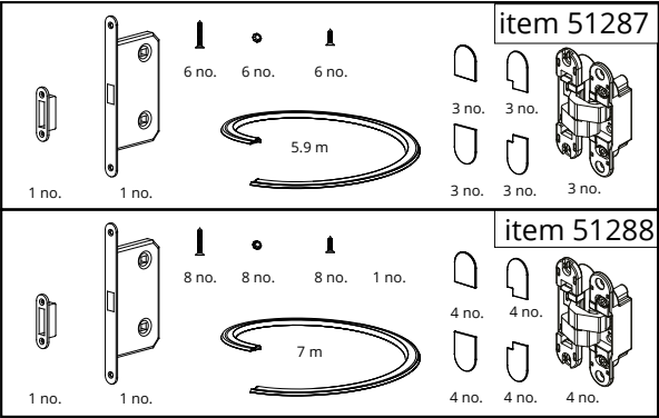
60 kg hinge set + magnet
