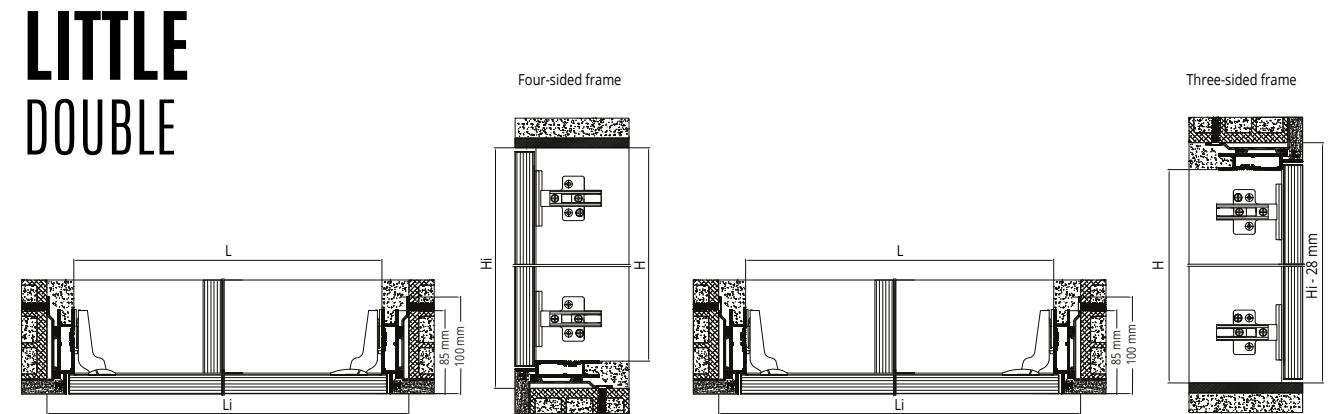
Double Door - Non-Std Size - Three-sided frame
