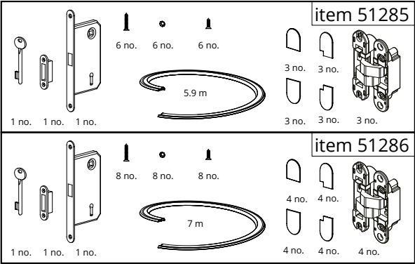
60 kg hinge set + Euro cylinder hole magnetic lock
