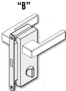
Handle with thumbturn and emergency release
